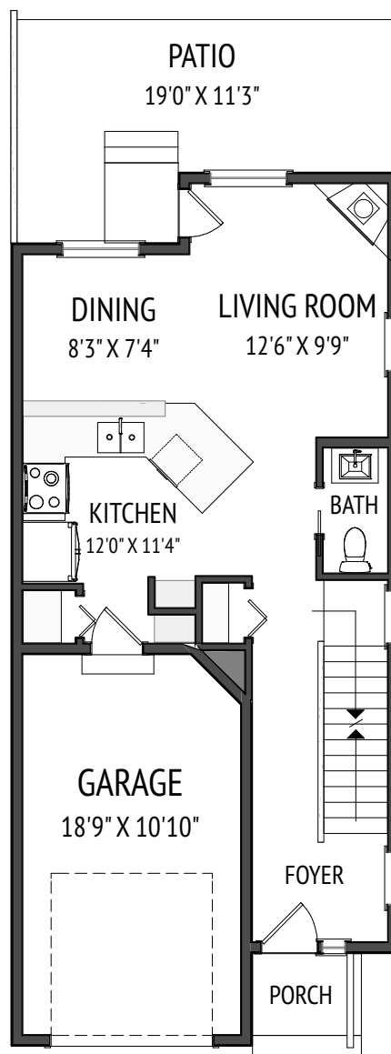
MAIN LEVEL
