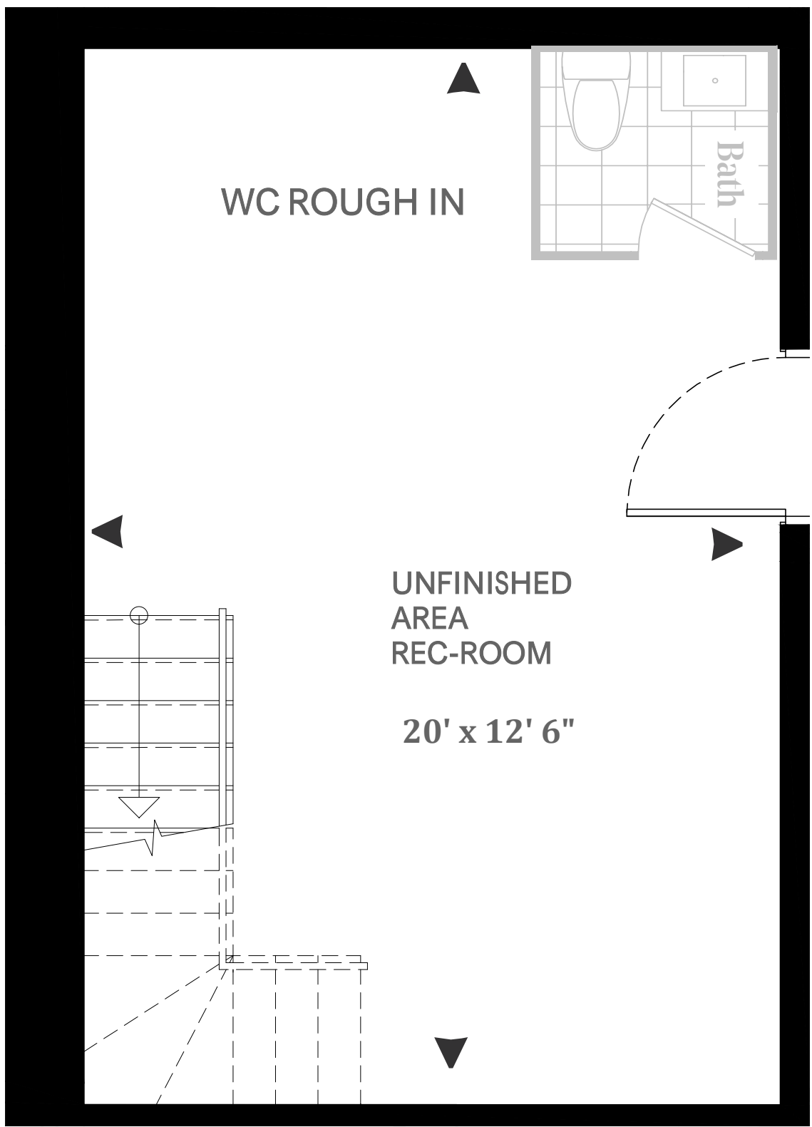
BASEMENT FLOOR
