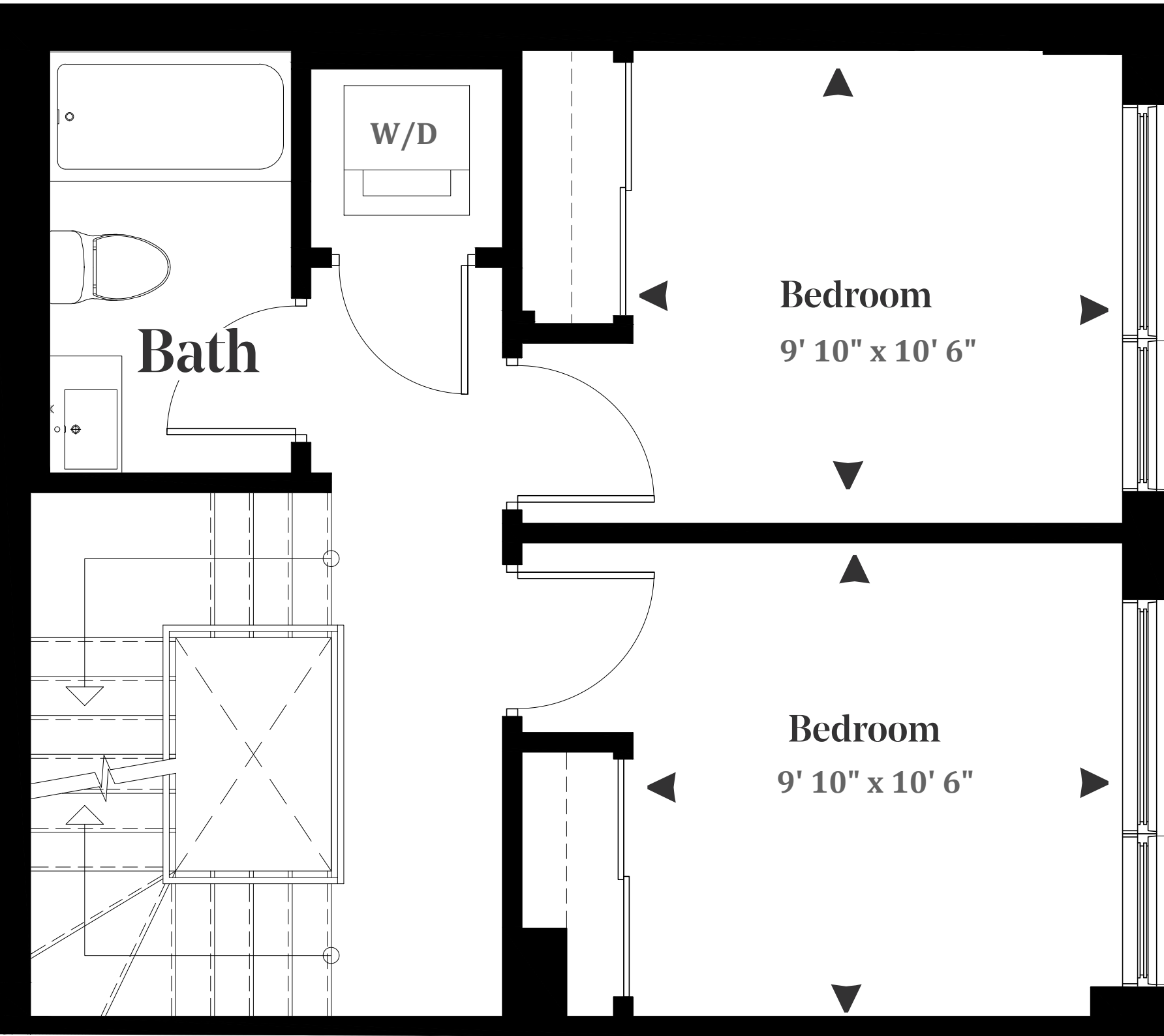
SECOND FLOOR
