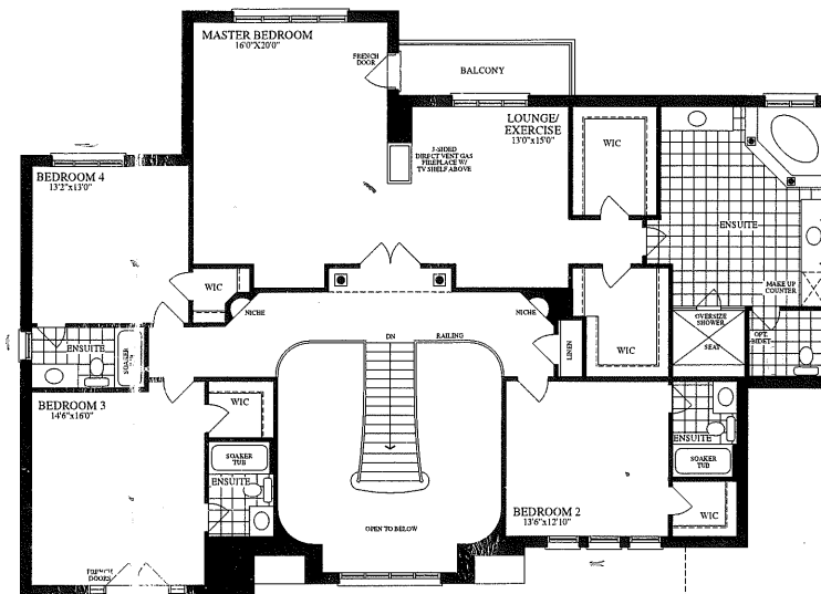
SECOND FLOOR 4 BEDROOM PLAN ELEVATION A
