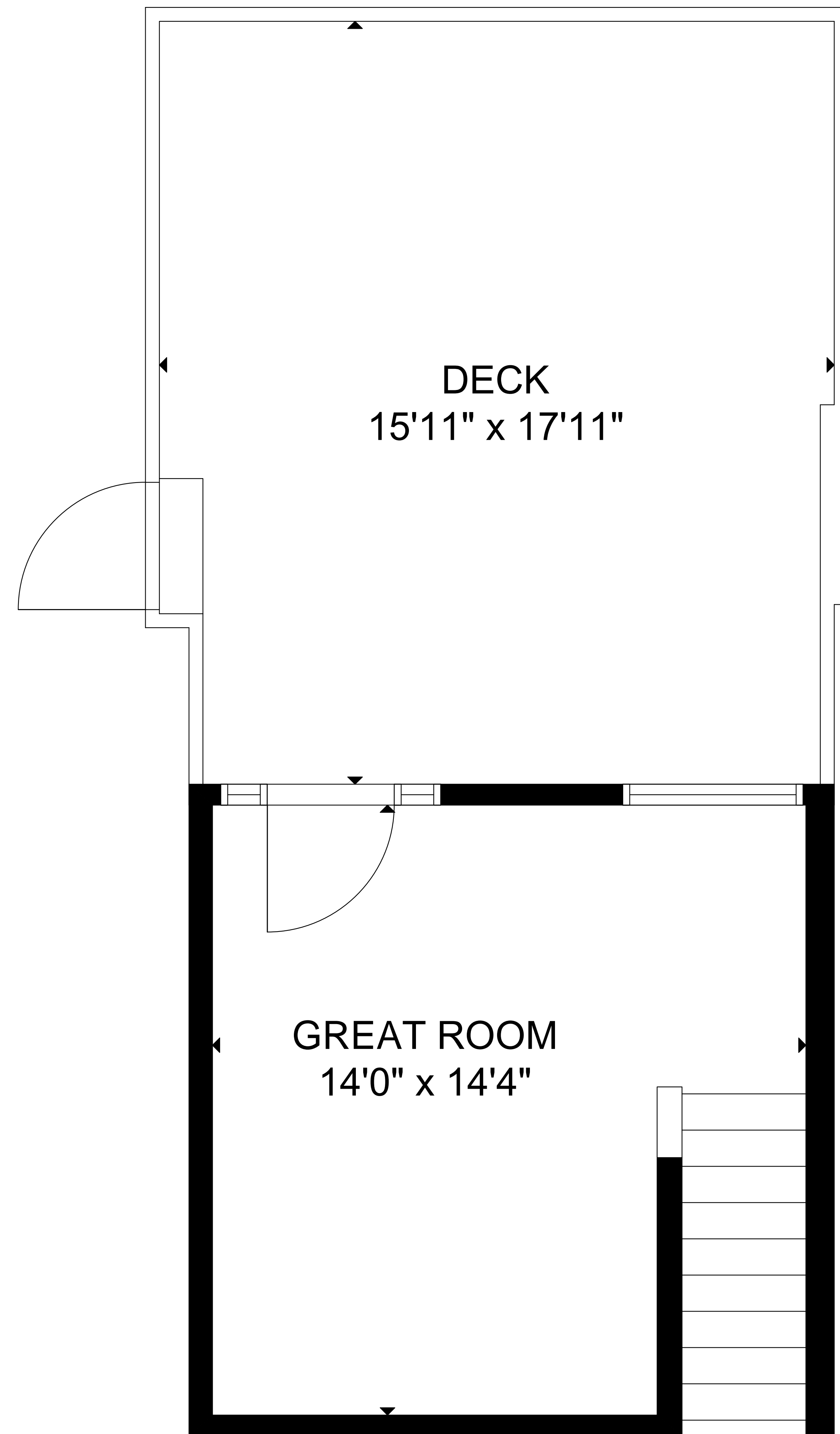
LOWER LEVEL
