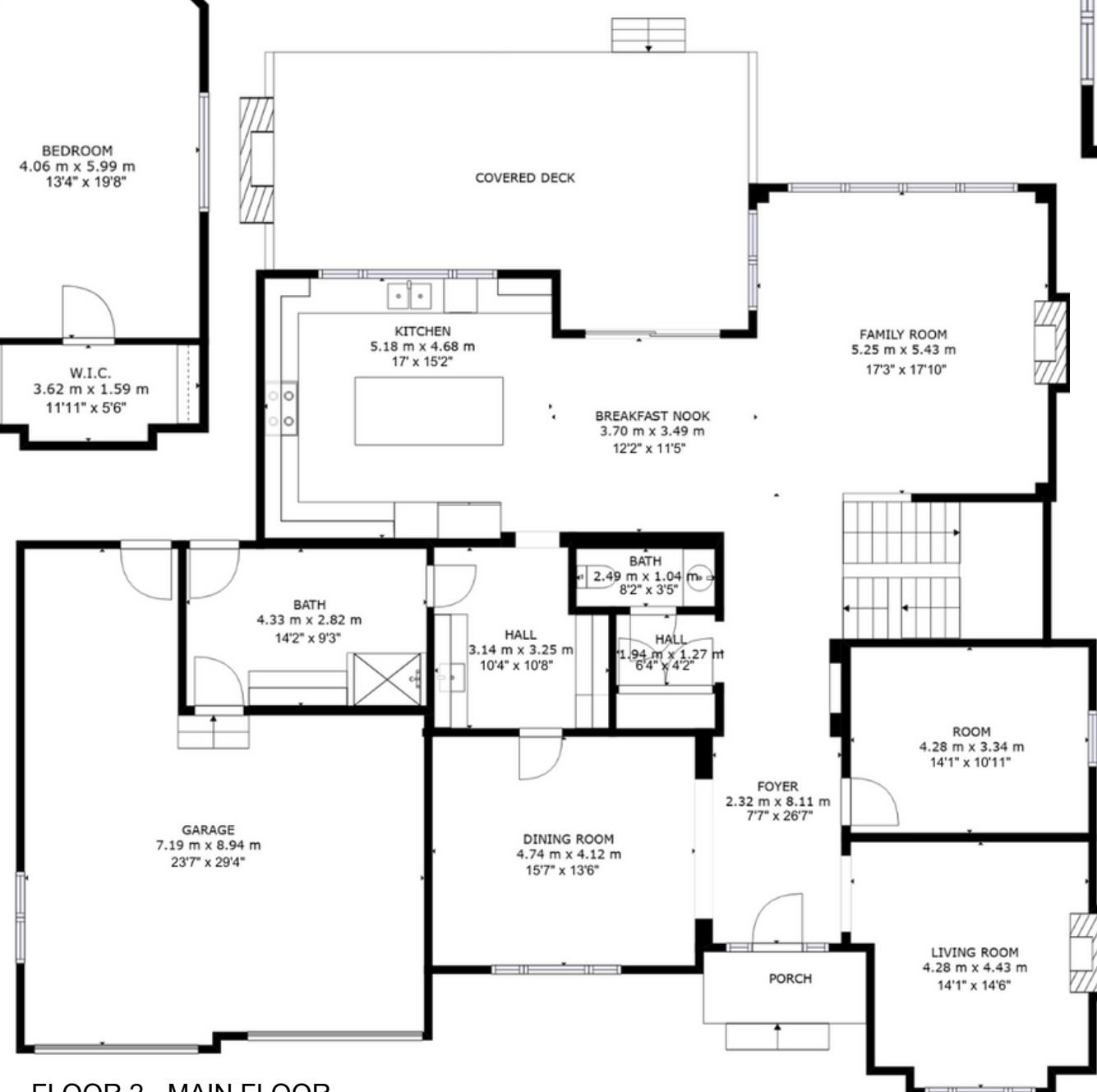
FLOOR 2 - MAIN FLOOR
